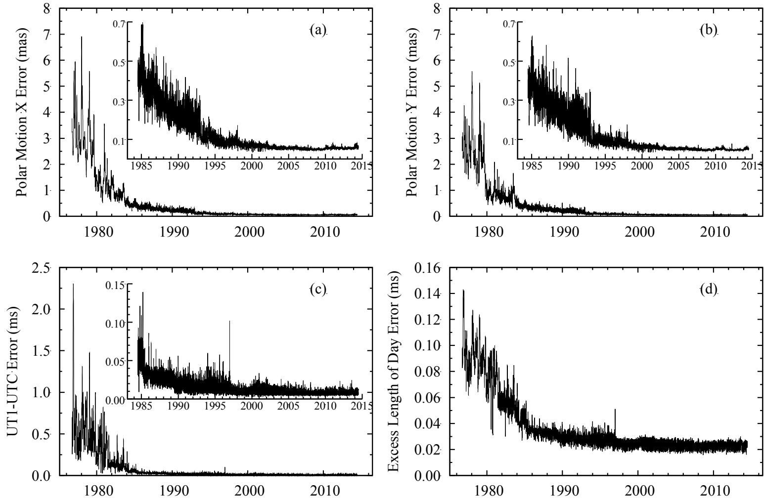
Figure 2. Plots of the 1\sigma formal errors of the x -component of polar motion (2a), y -component of polar motion (2b), UT1–UTC (2c), and excess length-of-day (2d) as given by the combined Earth orientation series SPACE2013. The inserts within panels (2a), (2b), and (2c) show that component’s post-1984 uncertainties on an expanded scale with the same units: milliarcseconds (mas) for polar motion, milliseconds (ms) for UT1–UTC.
