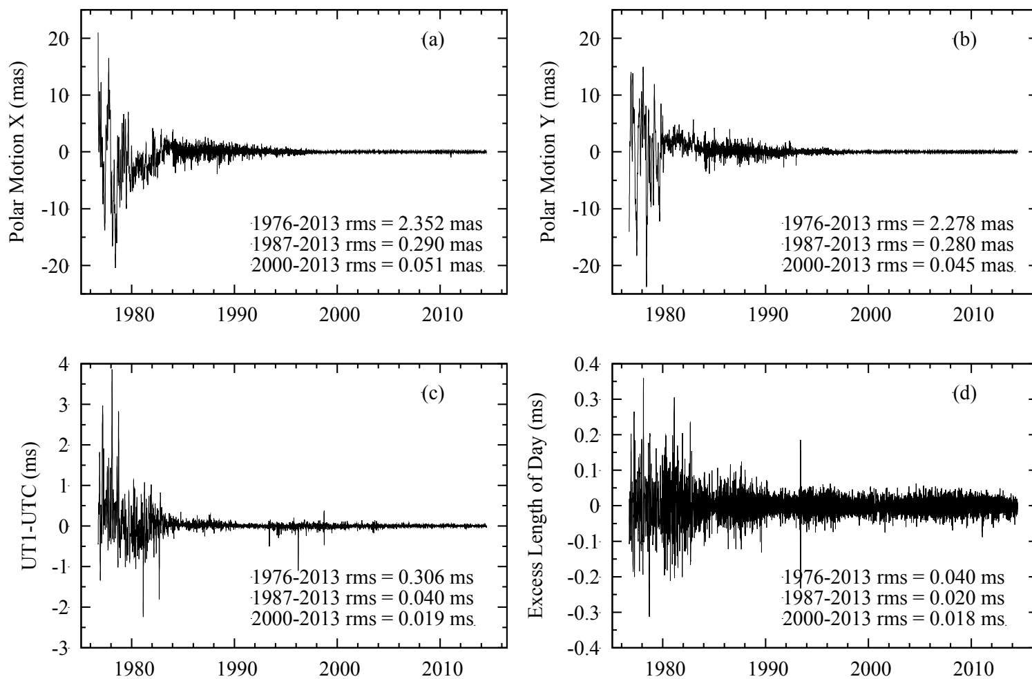
Figure 3. Plots of the difference between the IERS combined Earth orientation series EOP(IERS) 08 C 04 and SPACE2013 formed by subtracting the SPACE2013 values from those of the IERS series. The difference between the x -component of polar motion is shown in (3a), the difference between the y -component is shown in (3b), the difference between UT1-UTC is shown in (3c), and the difference between the excess length-of-day is shown in (3d).
