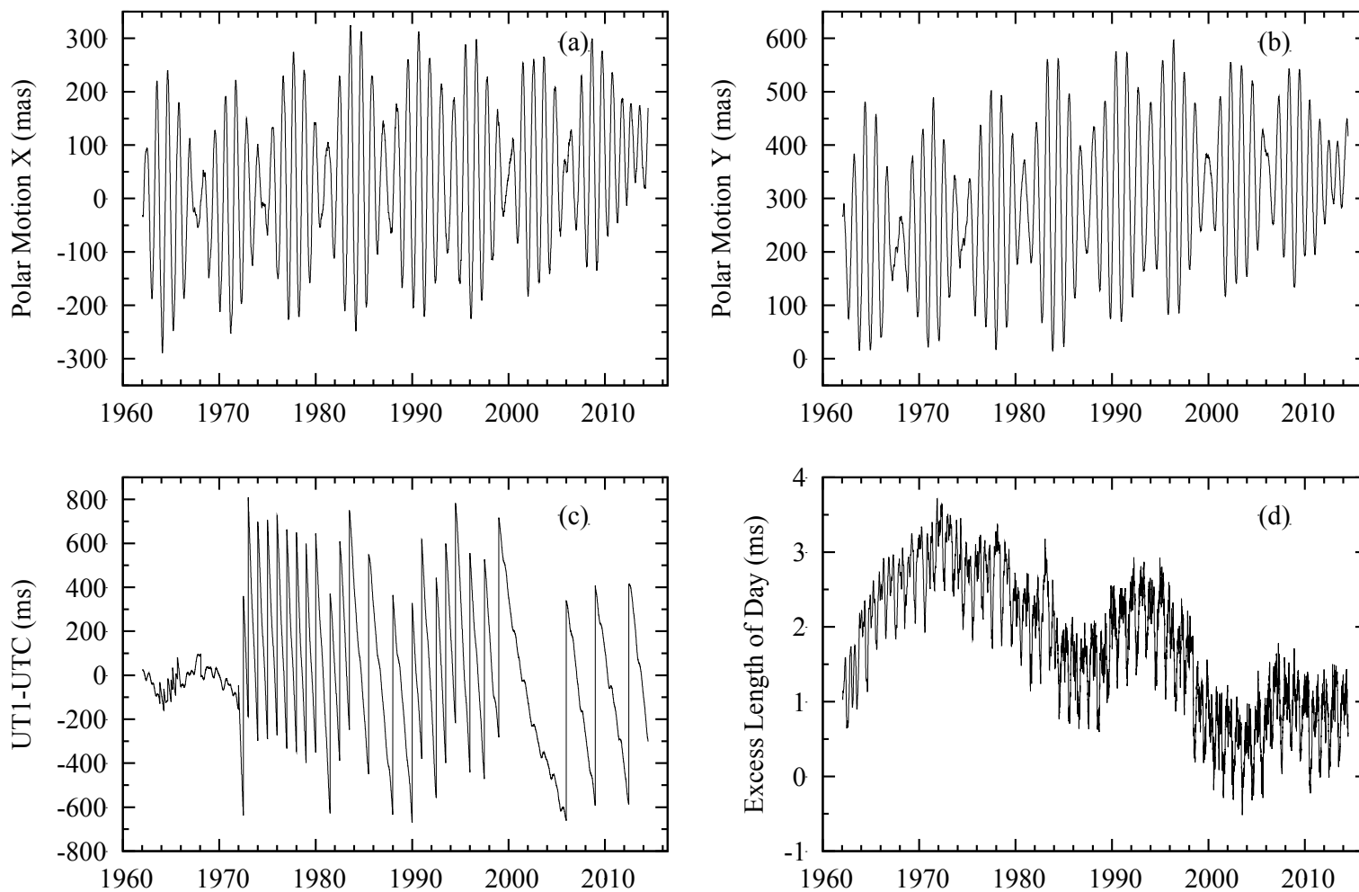
Figure 4. Plots of the x -component of polar motion (4a), y -component of polar motion (4b), UT1–UTC (4c), and excess length-of-day (4d) as given by the combined Earth orientation series, COMB2013. The discontinuous changes in the plot of UT1–UTC are caused by the presence of leap seconds. Prior to the introduction of leap seconds in 1972, Coordinated Universal Time (UTC) was adjusted by introducing step and rate changes designed to keep it close to UT1 (e.g., IERS 1997, Table II-3), the effect of which is also readily apparent in (4c). Note that the UT1–UTC values displayed in (4c) include the tidal variations, whereas the excess length-of-day values shown in (4d) do not.
