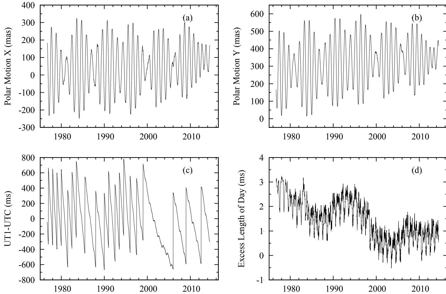
Figure 1. Plots of the x -component of polar motion (1a), y -component of polar motion (1b), UT1-UTC (1c), and excess length-of-day (1d) as given by the combined Earth orientation series SPACE2013. The discontinuous changes in the plot of UT1-UTC are caused by the presence of leap seconds. Note that the UT1-UTC values displayed in (1c) include the tidal variations, whereas the excess length-of-day values shown in (1d) do not.
