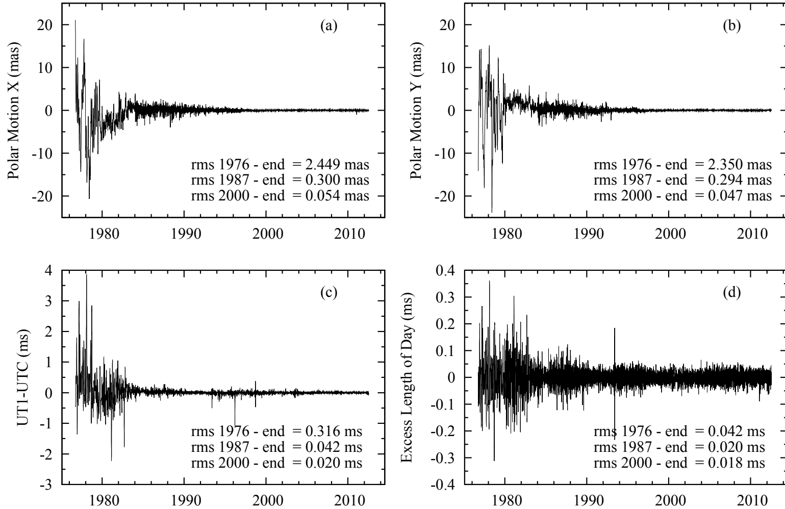
Figure 3. Plots of the difference between the IERS combined Earth orientation series EOP(IERS) 08 C 04 and SPACE2011 formed by subtracting the SPACE2011 values from those of the IERS series. The difference between the x -component of polar motion is shown in (3a), the difference between the y -component is shown in (3b), the difference between UT1–UTC is shown in (3c), and the difference between the excess length-of-day is shown in (3d).
