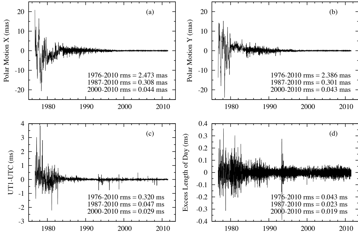
Figure 3. Plots of the difference between the IERS combined Earth orientation series EOP(IERS) 08 C 04 and SPACE2010 formed by subtracting the SPACE2010 values from those of the IERS series. The difference between the x -component of polar motion is shown in (3a), the difference between the y -component is shown in (3b), the difference between UT1-UTC is shown in (3c), and the difference between the excess length-of-day is shown in (3d).
