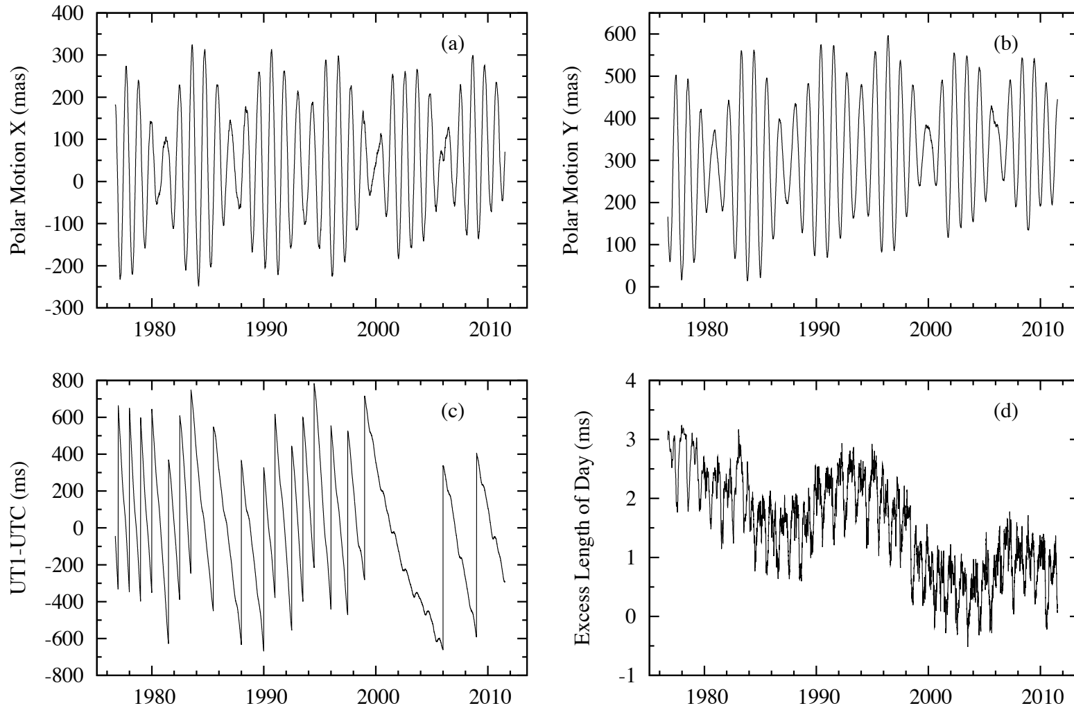
Figure 1. Plots of the x -component of polar motion (1a), y -component of polar motion (1b), UT1-UTC (1c), and excess length-of-day (1d) as given by the combined Earth orientation series SPACE2010. The discontinuous changes in the plot of UT1-UTC are caused by the presence of leap seconds. Note that the UT1-UTC values displayed in 1c include the tidal variations, whereas the excess length-of-day values shown in (1d) do not.
