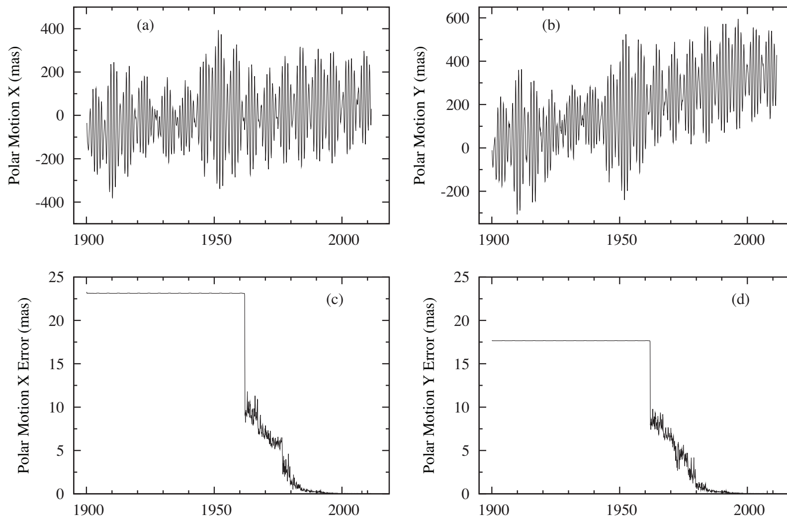
Figure 6. Plots of the x -component of polar motion (6a), the y -component of polar motion (6b), the 1\sigma formal errors of the x -component of polar motion (6c), and the 1\sigma formal errors of the y -component of polar motion (6d) as given by the combined polar motion series POLE2010.
