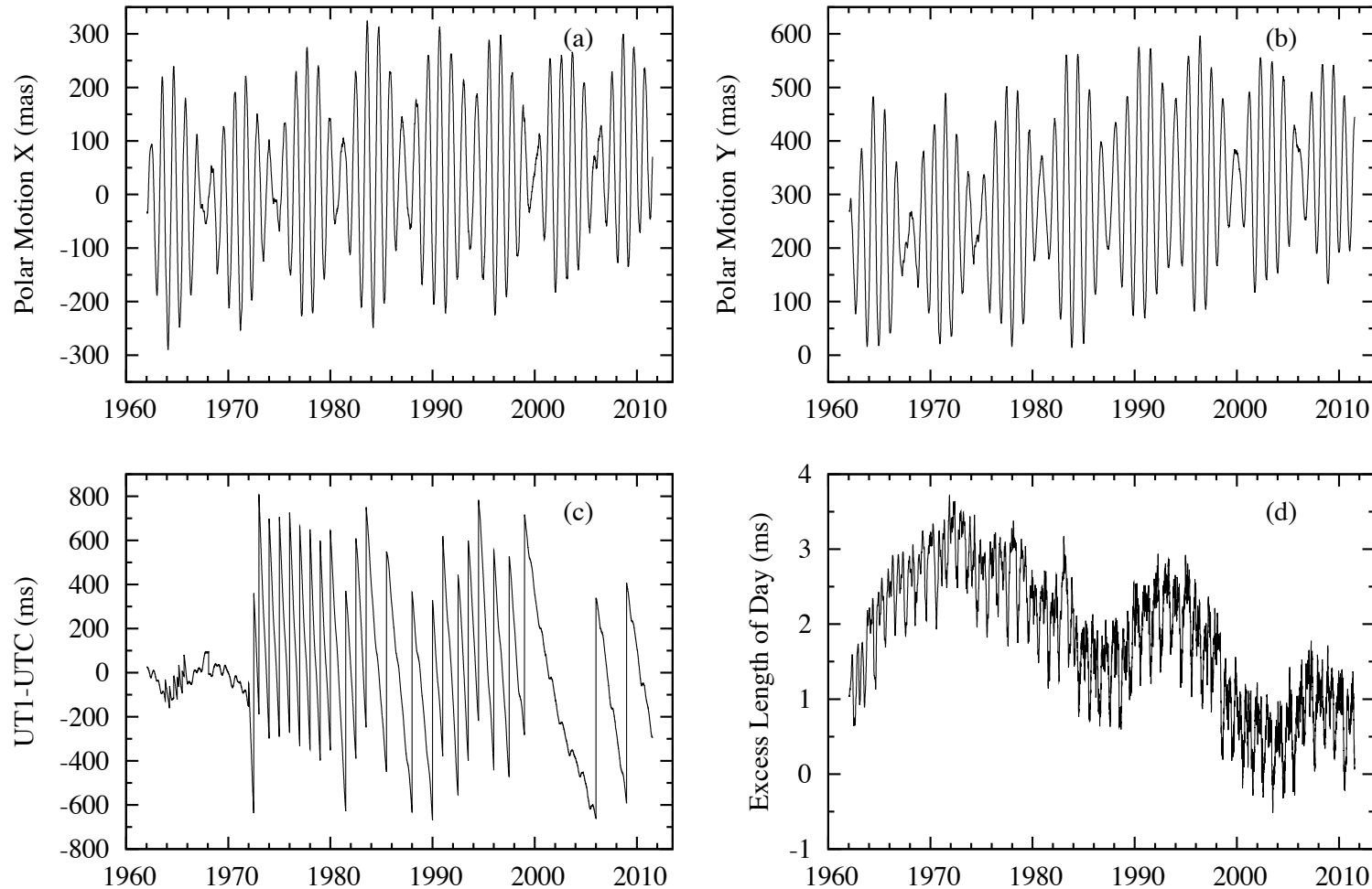
Figure 4. Plots of the x -component of polar motion (4a), y -component of polar motion (4b), UT1–UTC (4c), and excess length-of-day (4d) as given by the combined Earth orientation series, COMB2010. The discontinuous changes in the plot of UT1–UTC are caused by the presence of leap seconds. Prior to the introduction of leap seconds in 1972, Coordinated Universal Time (UTC) was adjusted by introducing step and rate changes designed to keep it close to UT1 (e.g., IERS 1997, Table II-3), the effect of which is also readily apparent in (4c). Note that the UT1–UTC values displayed in (4c) include the tidal variations, whereas the excess length-of-day values shown in (4d) do not.
