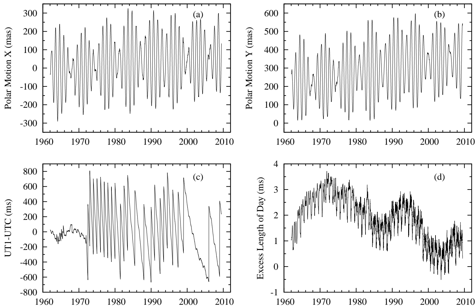
Figure 4. Plots of the x -component of polar motion (4a), y -component of polar motion (4b), UT1–UTC (4c), and excess length-of-day (4d) as given by the combined Earth orientation series, COMB2008. The discontinuous changes in the plot of UT1–UTC are caused by the presence of leap seconds. Prior to the introduction of leap seconds in 1972, Coordinated Universal Time (UTC) was adjusted by introducing step and rate changes designed to keep it close to UT1 (e.g., IERS 1997, Table II-3), the effect of which is also readily apparent in 4c. Note that the UT1–UTC values displayed in 4c include the tidal variations, whereas the excess length-of-day values shown in 4d do not.
