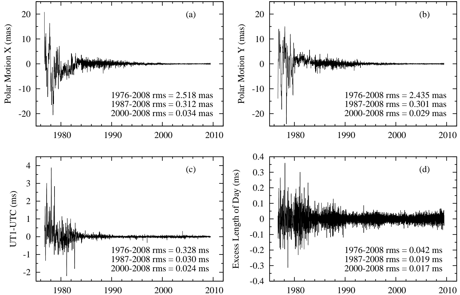
Figure 3. Plots of the difference between the IERS combined Earth orientation series EOP(IERS) 05 C 04 and SPACE2008 formed by subtracting the SPACE2008 values from those of the IERS series. The difference between the x -component of polar motion is shown in 3a, the difference between the y -component is shown in 3b, the difference between UT1–UTC is shown in 3c, and the difference between the excess length-of-day is shown in 3d.
