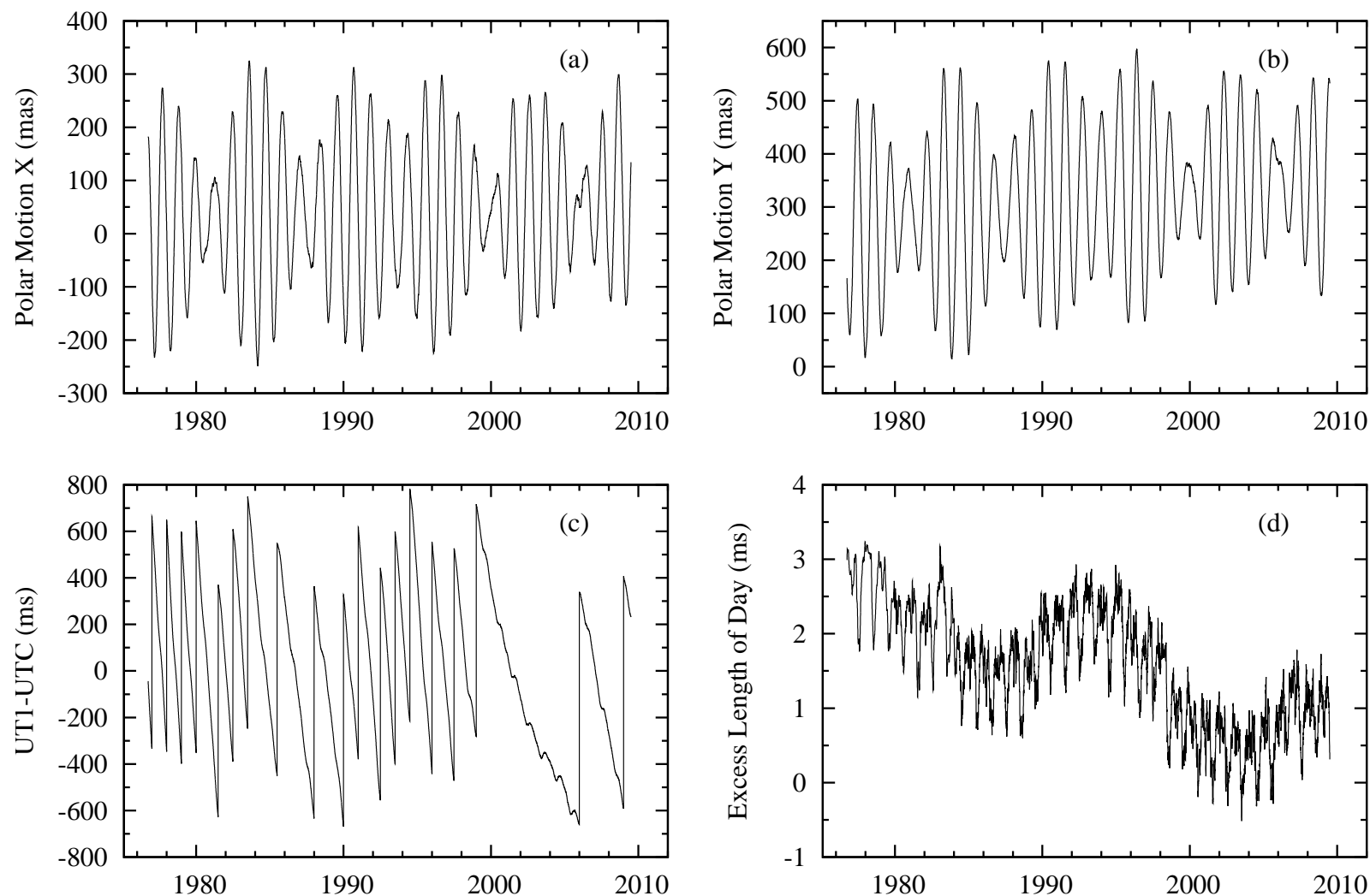
Figure 1. Plots of the x -component of polar motion (1a), y -component of polar motion (1b), UT1–UTC (1c), and excess length-of-day (1d) as given by the combined Earth orientation series SPACE2008. The discontinuous changes in the plot of UT1–UTC are caused by the presence of leap seconds. Note that the UT1–UTC values displayed in 1c include the tidal variations, whereas the excess length-of-day values shown in 1d do not.
