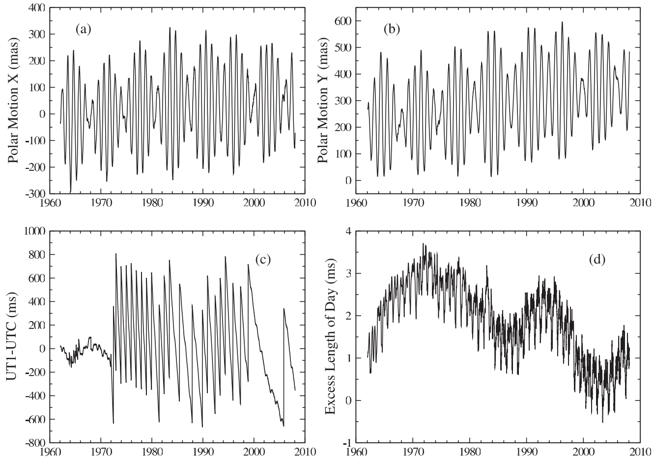
Figure 4. Plots of the x -component of polar motion (4a), y -component of polar motion (4b), UT1–UTC (4c), and excess length-of-day (4d) as given by the combined Earth orientation series, COMB2007. The discontinuous changes in the plot of UT1–UTC are caused by the presence of leap seconds. Prior to the introduction of leap seconds in 1972, Coordinated Universal Time (UTC) was adjusted by introducing step and rate changes designed to keep it close to UT1 (e.g., IERS 1997, Table II-3), the effect of which is also readily apparent in 4c. Note that the UT1–UTC values displayed in 4c include the tidal variations, whereas the excess length-of-day values shown in 4d do not.
