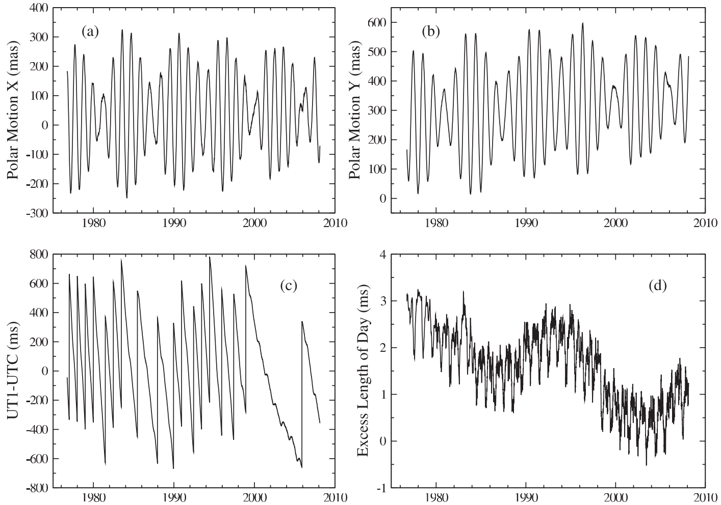
Figure 1. Plots of the x -component of polar motion (1a), y -component of polar motion (1b), UT1-UTC (1c), and excess length-of-day (1d) as given by the combined Earth orientation series SPACE2007. The discontinuous changes in the plot of UT1-UTC are caused by the presence of leap seconds. Note that the UT1-UTC values displayed in 1c include the tidal variations, whereas the excess length-of-day values shown in 1d do not.
