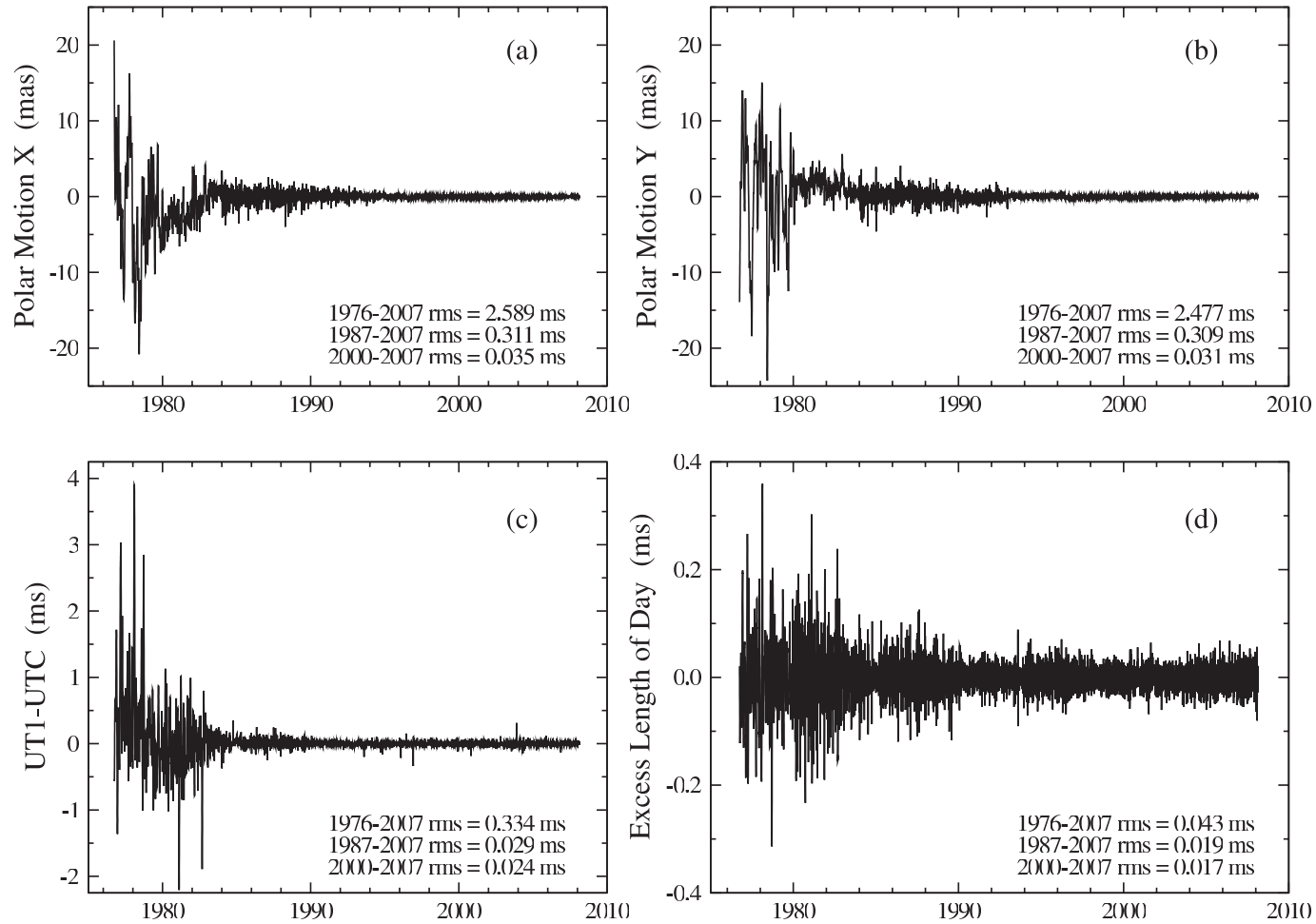
Figure 3. Plots of the difference between the IERS combined Earth orientation series EOP(IERS) 05 C 04 and SPACE2007 formed by subtracting the SPACE2007 values from those of the IERS series. The difference between the x -component of polar motion is shown in 3a, the difference between the y -component is shown in 3b, the difference between UT1–UTC is shown in 3c, and the difference between the excess length-of-day is shown in 3d.
