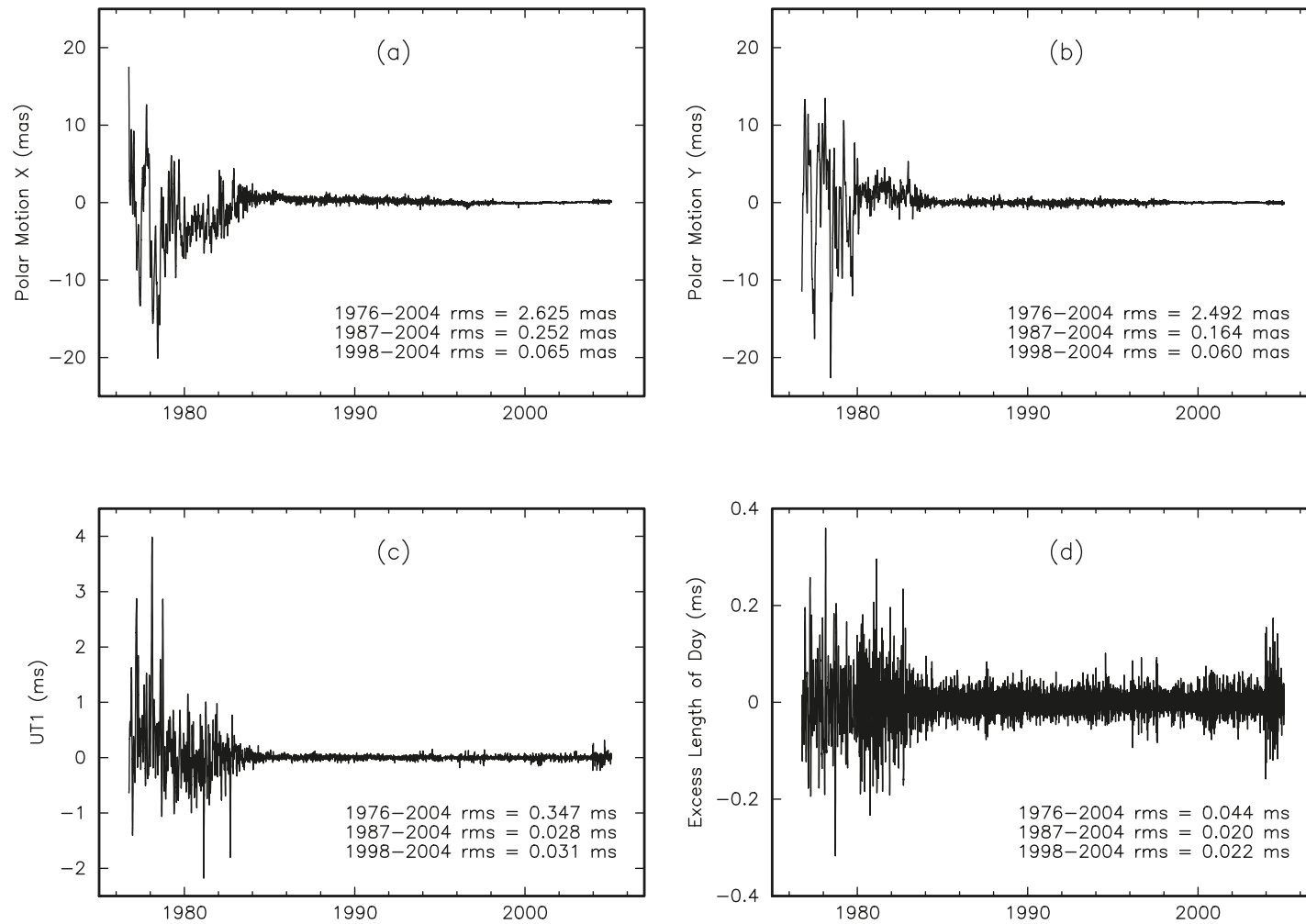
Figure 3. Plots of the difference between the IERS combined Earth orientation series EOP(IERS) C 04 and SPACE2004 formed by subtracting the SPACE2004 values from those of the IERS series. The difference between the x -component of polar motion is shown in 3a, the difference between the y -component is shown in 3b, the difference between UT1-UTC is shown in 3c, and the difference between the excess length-of-day is shown in 3d.
