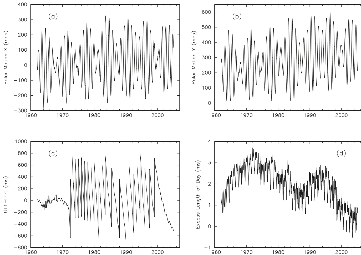
Figure 4. Plots of the x -component of polar motion (4a), y -component of polar motion (4b), UT1-UTC (4c), and excess length-of-day (4d) as given by the combined Earth orientation series, COMB2004. The discontinuous changes in the plot of UT1-UTC are caused by the presence of leap seconds. Prior to the introduction of leap seconds in 1972, Coordinated Universal Time (UTC) was adjusted by introducing step and rate changes designed to keep it close to UT1 (e.g., IERS 1997, Table II-3), the effect of which is also readily apparent in 4c. Note that the UT1-UTC values displayed in 4c include the tidal variations, whereas the excess length-of-day values shown in 4d do not.
