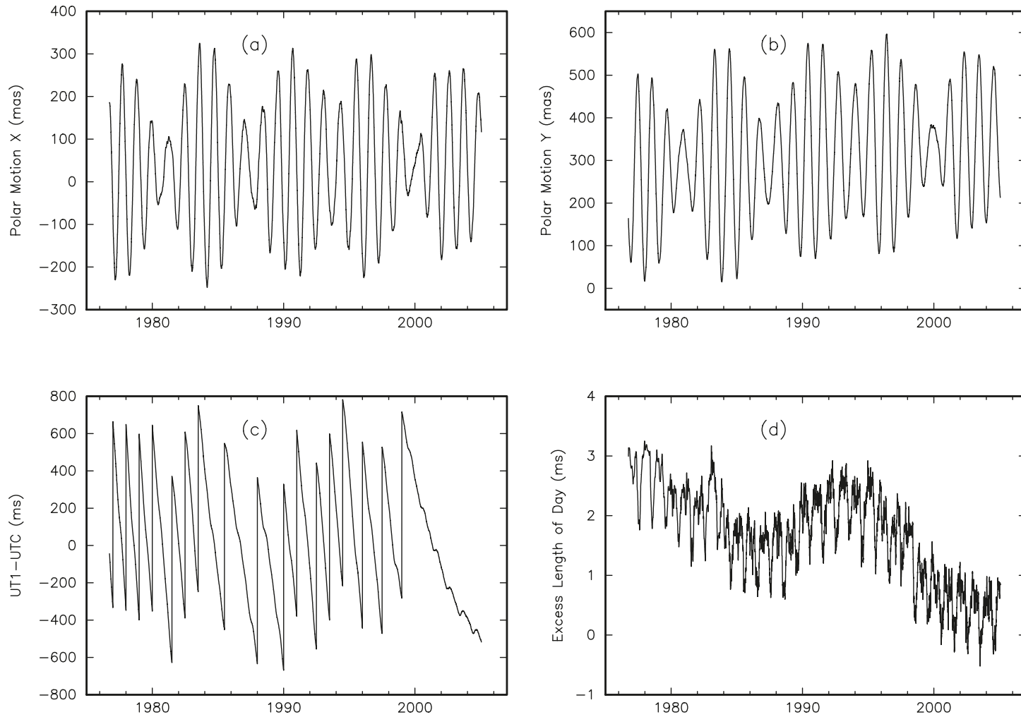
Figure 1. Plots of the x -component of polar motion (1a), y -component of polar motion (1b), UT1-UTC (1c), and excess length-of-day (1d) as given by the combined Earth orientation series SPACE2004. The discontinuous changes in the plot of UT1-UTC are caused by the presence of leap seconds. Note that the UT1-UTC values displayed in 1c include the tidal variations, whereas the excess length-of-day values shown in 1d do not.
