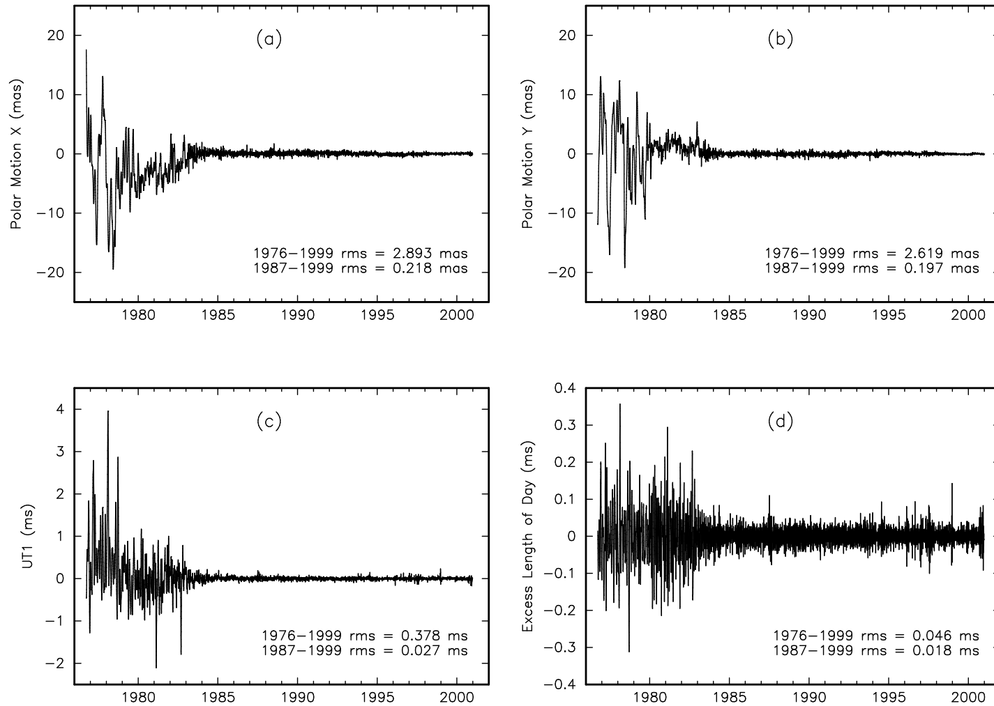
Figure 3. Plots of the difference between the IERS combined Earth orientation series EOP(IERS) C 04 and SPACE2000 formed by subtracting the SPACE2000 values from those of the IERS series. The difference between the x component of polar motion is shown in 3a, the difference between the y component is shown in 3b, the difference between UT1-UTC is shown in 3c, and the difference between the excess length of day is shown in 3d.
