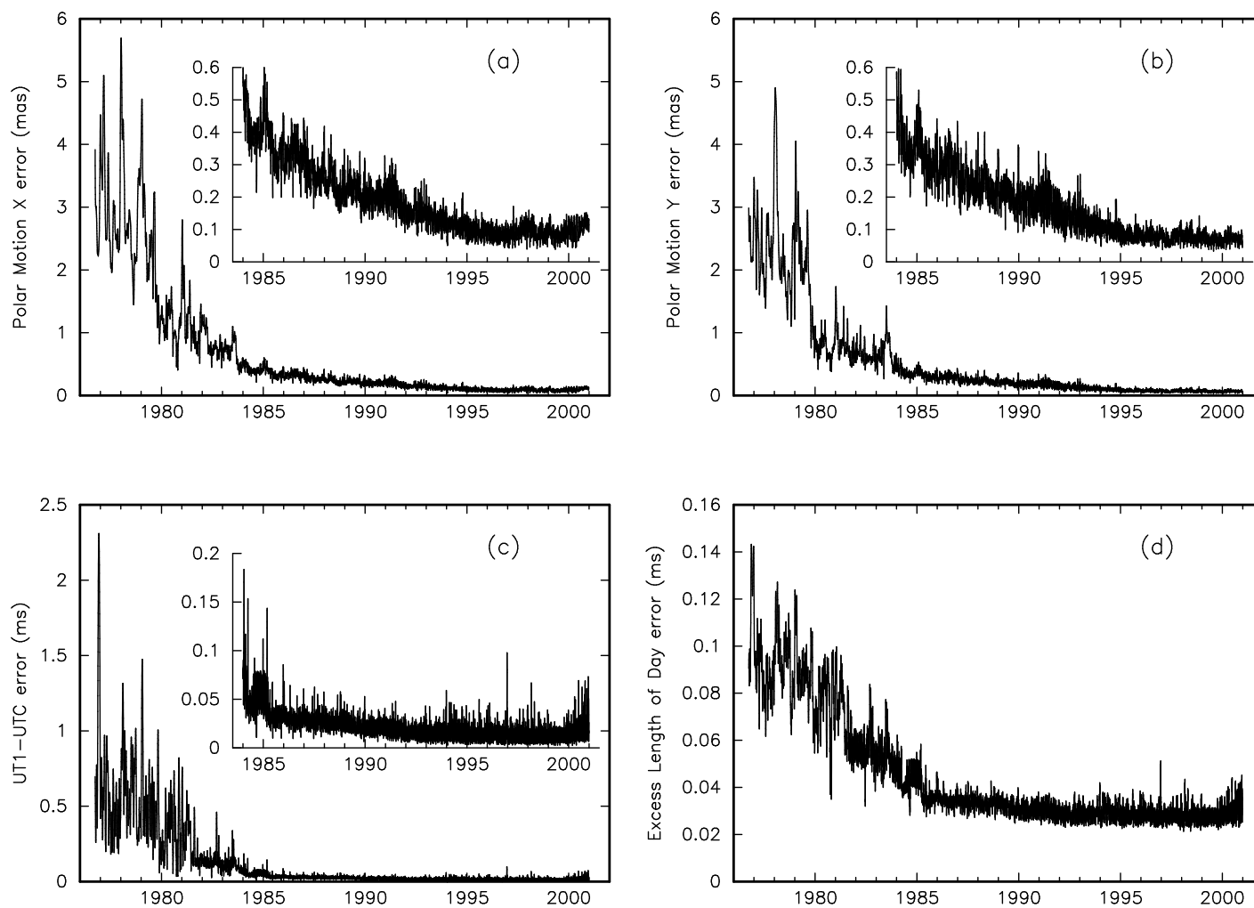
Figure 2. Plots of the 1 \sigma formal errors of the x component of polar motion (2a), the y component of polar motion (2b), UT1–UTC (2c), and excess length of day (2d) as given by the combined Earth orientation series SPACE2000. The insert within panels 2a, 2b, and 2c shows that component’s post-1984 uncertainties on an expanded scale with the same units: milliarcseconds (mas) for polar motion; milliseconds (ms) for UT1–UTC.
