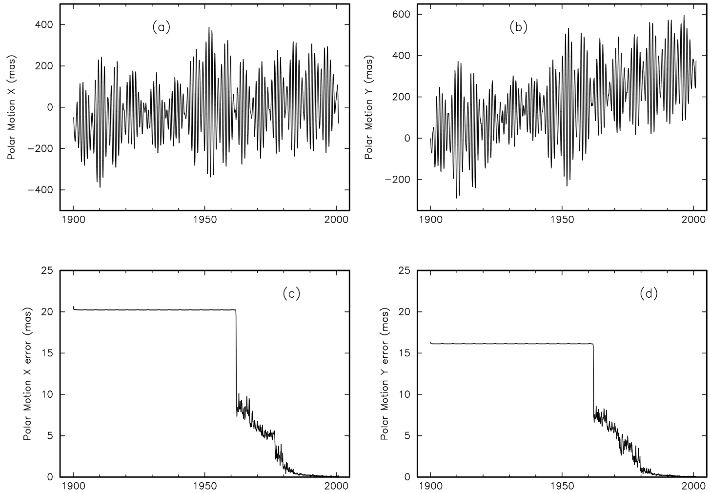
Figure 6. Plots of the x component of polar motion (6a), the y component of polar motion (6b), the 1\text{-}\sigma formal errors of the x component of polar motion (6c), and the 1\text{-}\sigma formal errors of the y component of polar motion (6d) as given by the combined polar motion series POLE2000.
