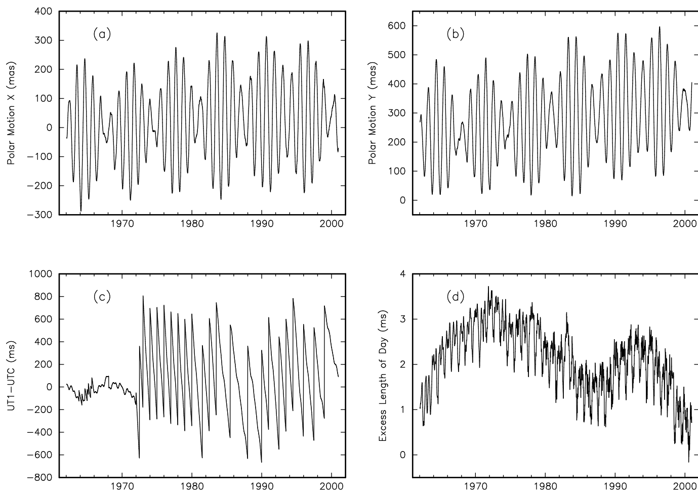
Figure 4. Plots of the x component of polar motion (4a), the y component of polar motion (4b), UT1-UTC (4c), and excess length of day (4d) as given by the combined Earth orientation series COMB2000. The discontinuous changes in the plot of UT1-UTC are caused by the presence of leap seconds. Prior to the introduction of leap seconds in 1972, Coordinated Universal Time (UTC) was adjusted by introducing step and rate changes designed to keep it close to UT1 (e.g., IERS 2000, Table IV-3), the effect of which is also readily apparent in 4c. Note that the UT1-UTC values displayed in 4c include the tidal variations, whereas the excess length-of-day values shown in 4d do not.
