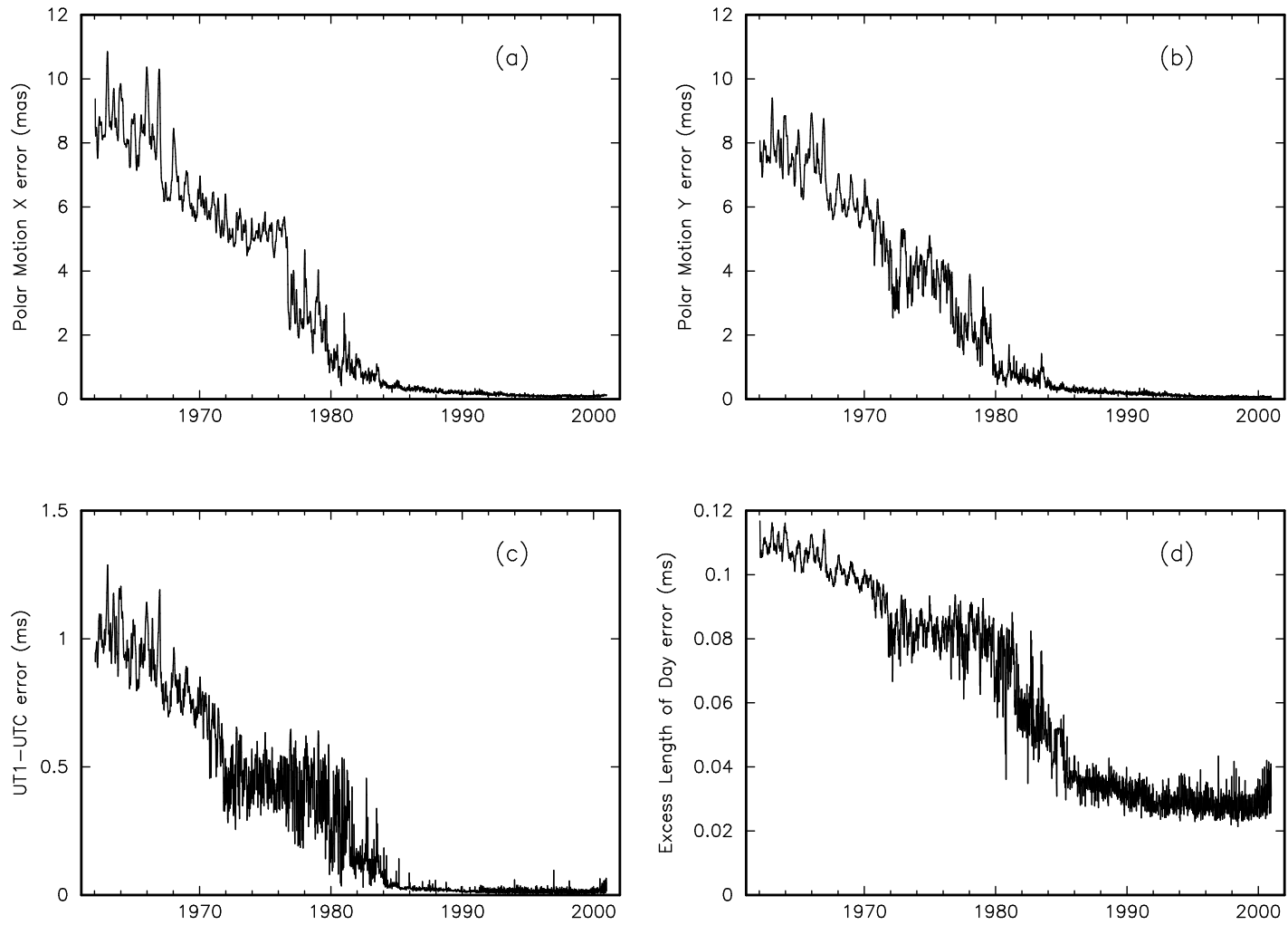
Figure 5. Plots of the 1 formal errors of the x component of polar motion (5a), the y component of polar motion (5b), UT1-UTC (5c), and excess length of day (5d) as given by the combined Earth orientation series COMB2000.
