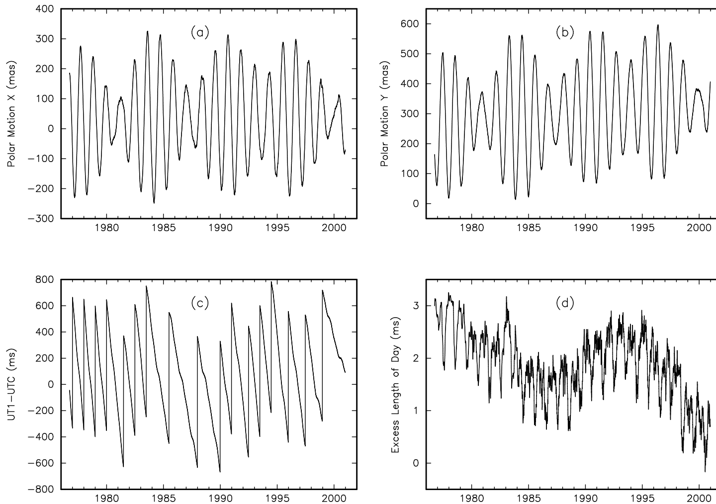
Figure 1. Plots of the x component of polar motion (1a), the y component of polar motion (1b), UT1-UTC (1c), and excess length of day (1d) as given by the combined Earth orientation series SPACE2000. The discontinuous changes in the plot of UT1-UTC are caused by the presence of leap seconds. Note that the UT1-UTC values displayed in 1c include the tidal variations, whereas the excess length-of-day values shown in 1d do not.
